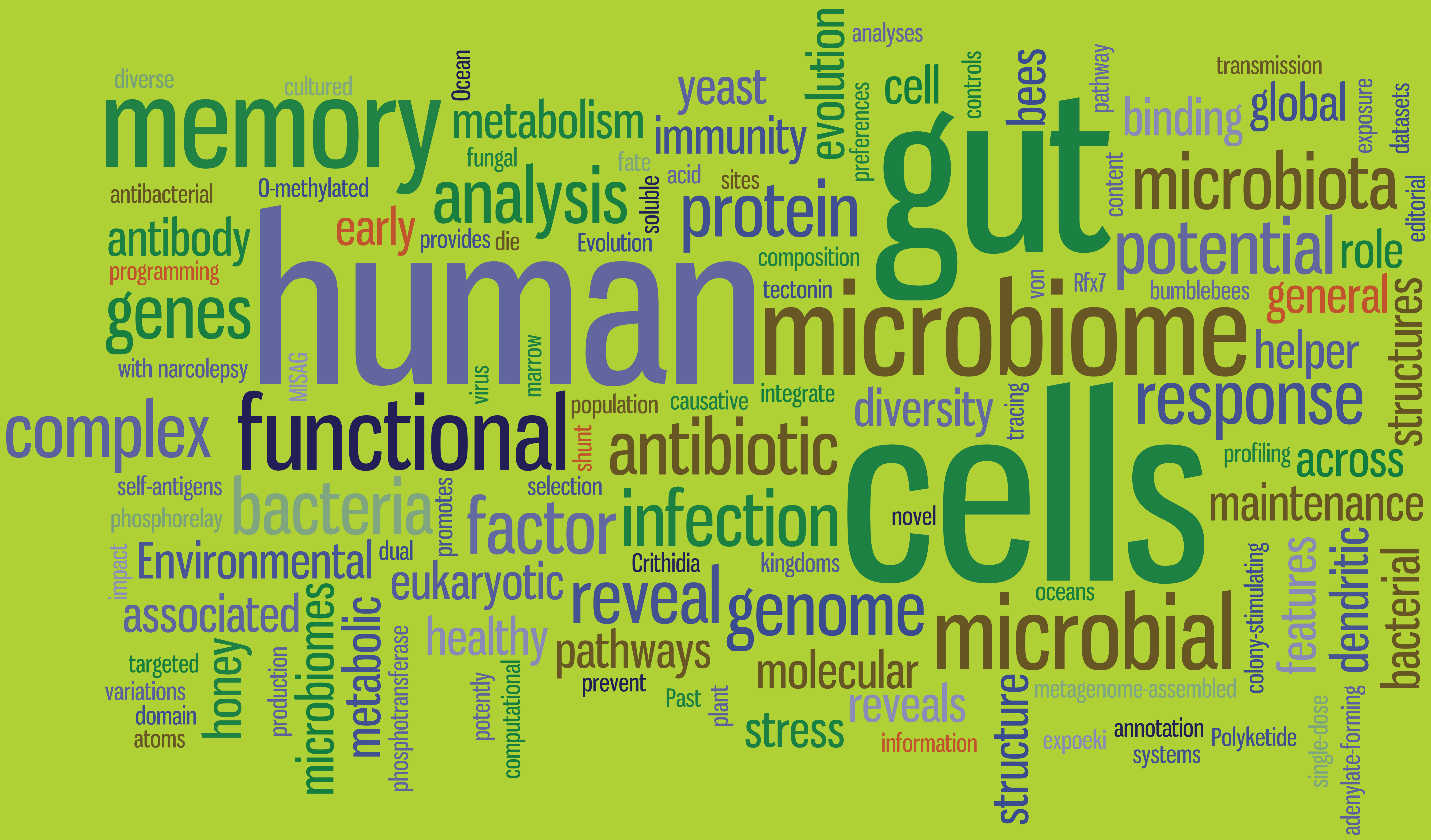
Scientific Publications of the Institute of Microbiology in 2018. Title word cloud designed by Chemistry | Biology | Pharmacy Information Center, ETH Zürich, using Scopus Author Search and Wordle.
